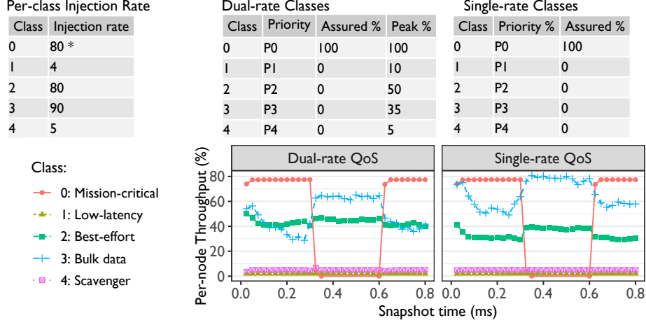
Fig. 6. Change in class throughput over time as mission critical traffic is transferred. *The mission-critical job suspends sending traffic at 0.3ms and resumes at 0.6ms. Workload and traffic-to-class assignments details are provided in Table 2. Traffic in class 2 (best effort) is able to sustain higher throughput with the dual-rate solution, even when the mission critical traffic is present.
